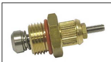
VALVOLA FERRO Vap-Vap VALVE All-Steam Iron VANNE FER Vap-Vap
